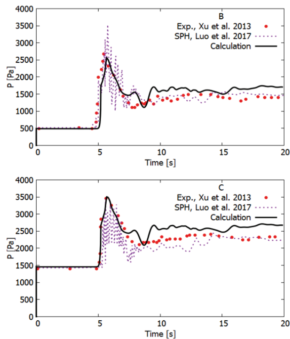
Figure 7. Pressure profiles at measurement points B and C.
