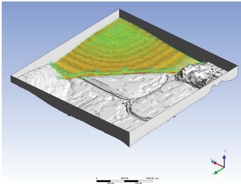
Figure 12. Setup of the real three-dimensional problem.
