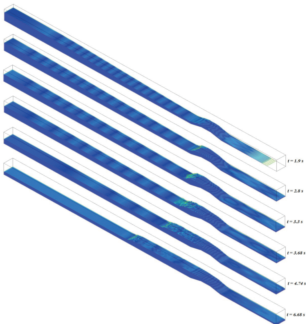
Figure 4. Three-dimensional wave contours at different time moments.
