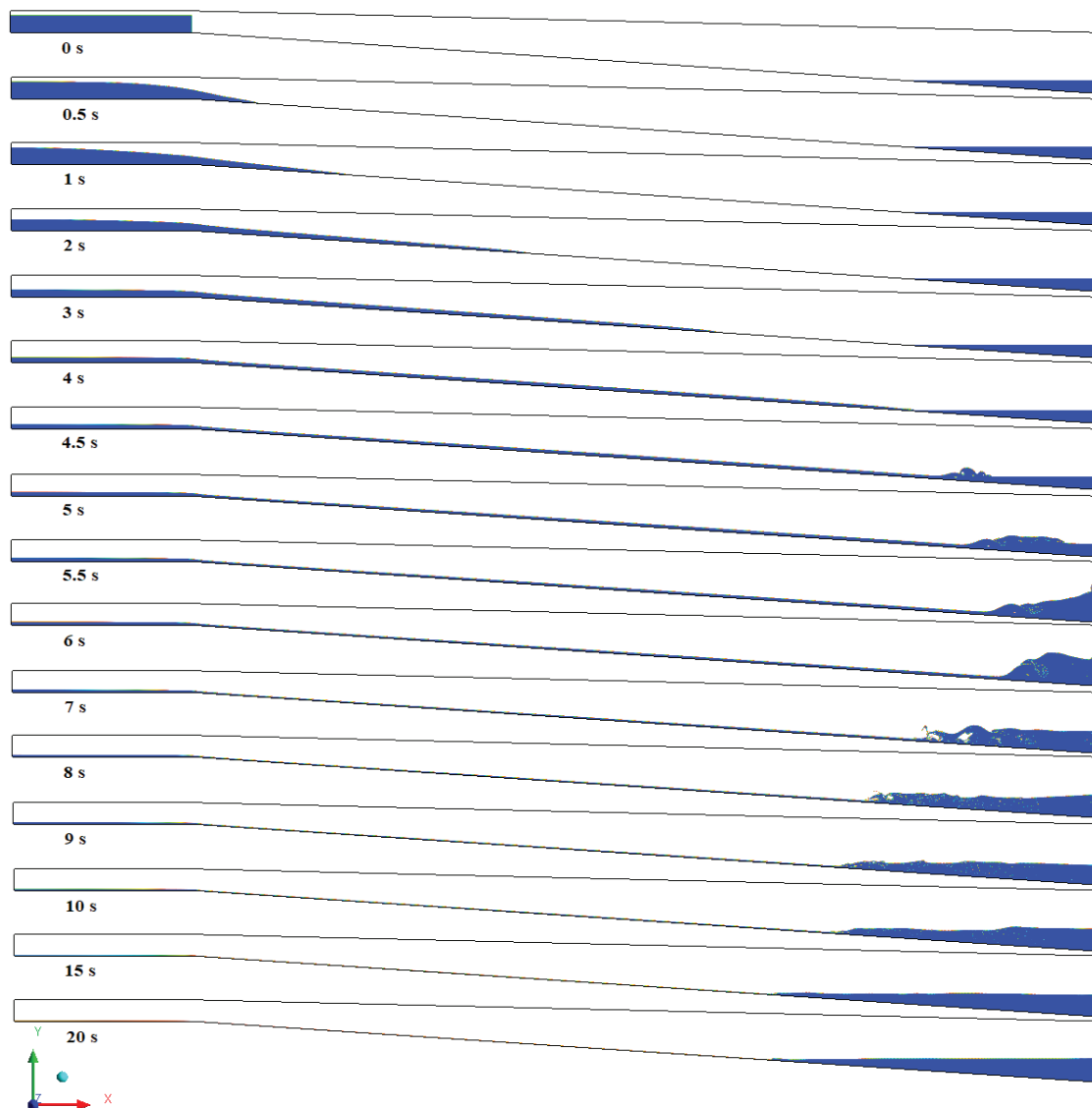
Figure 8. Snapshots of the dam break at different time moments.
