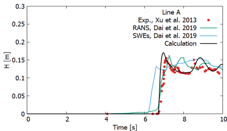
Figure 6. Water level along measurement line A at different time moments.
