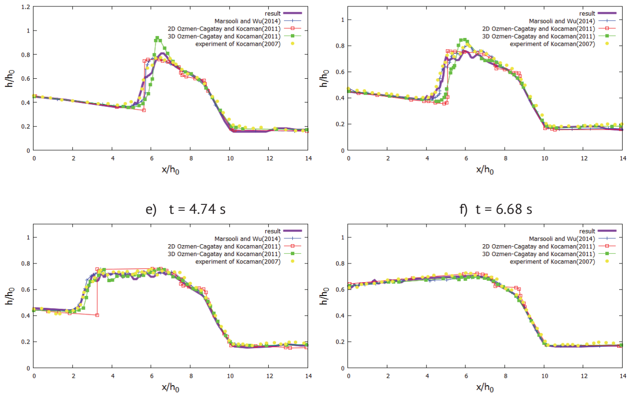
Figure 2. Water level height graphs at different time moments.
