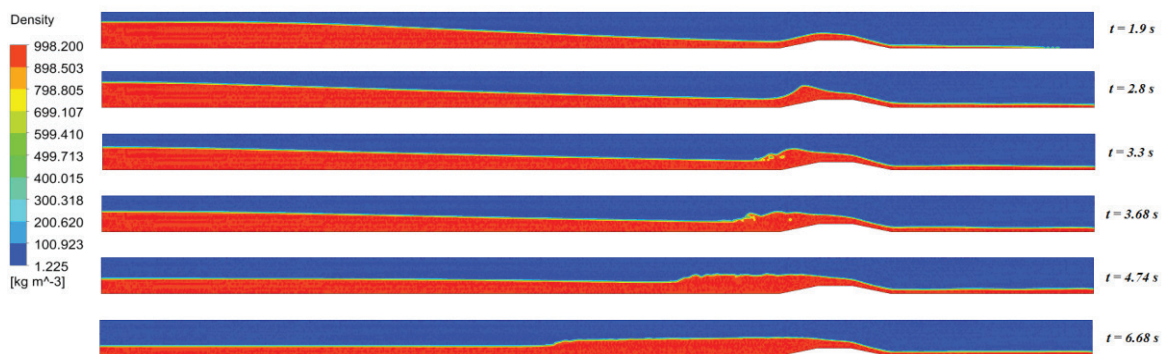
Figure 3. Two-dimensional wave contours.
