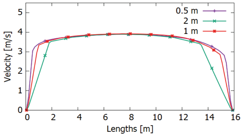
Figure 13. Velocity profiles in the Chu River for the different mesh sizes..
