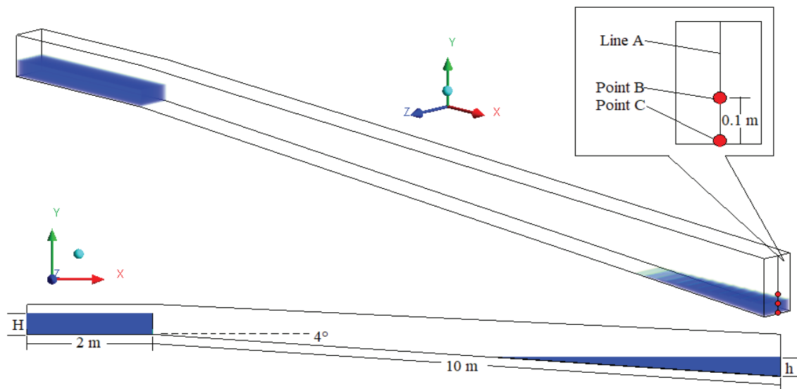
Figure 5. Geometry of the experimental setup with inclination.
