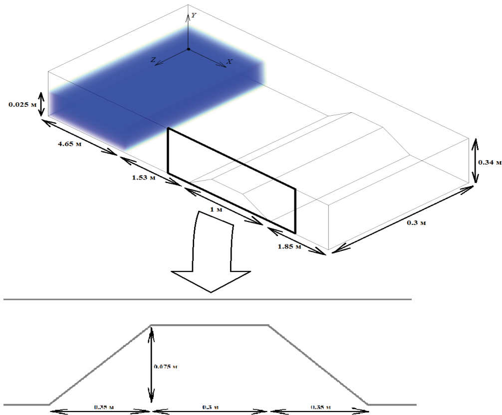
Figure 1. Geometry of the first test case with a trapezoidal step.
