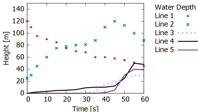
Figure 15. Flow height profiles at the measurement lines.
