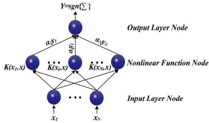
Figure 3. Structural diagram of information in the support vector method [4]
