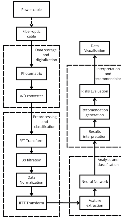
Figure 5. Conceptual model of the intellectual system
