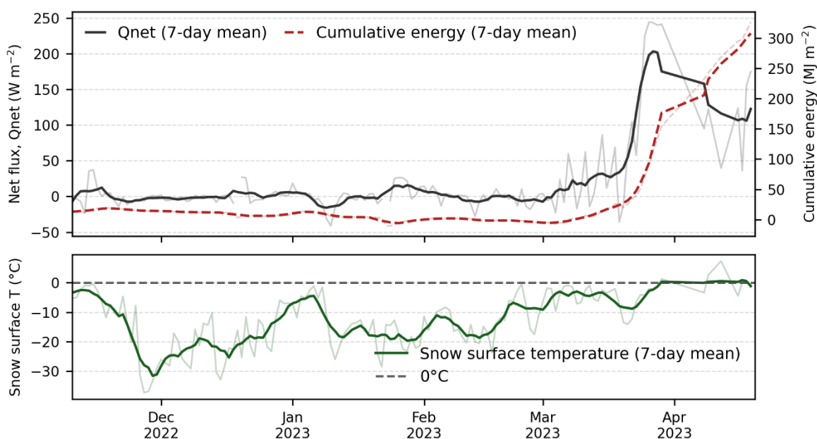
Figure 8. Net surface energy flux ( Q_{net} ), cumulative surface energy, and snow surface temperature during the 2022–2023 snow season. Melt periods coincide with rapid energy accumulation and surface temperature approaching 0\text{ }^{\circ}\text{C} , indicating energy-balance control.
