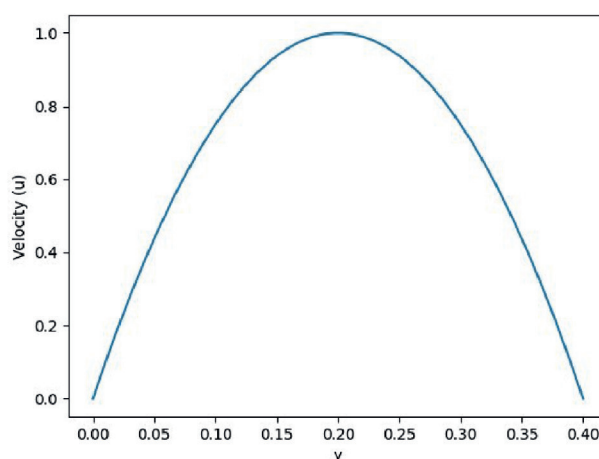
Figure 3. Input values of u along the y axis at x = 0 at a parabolic constant flow
