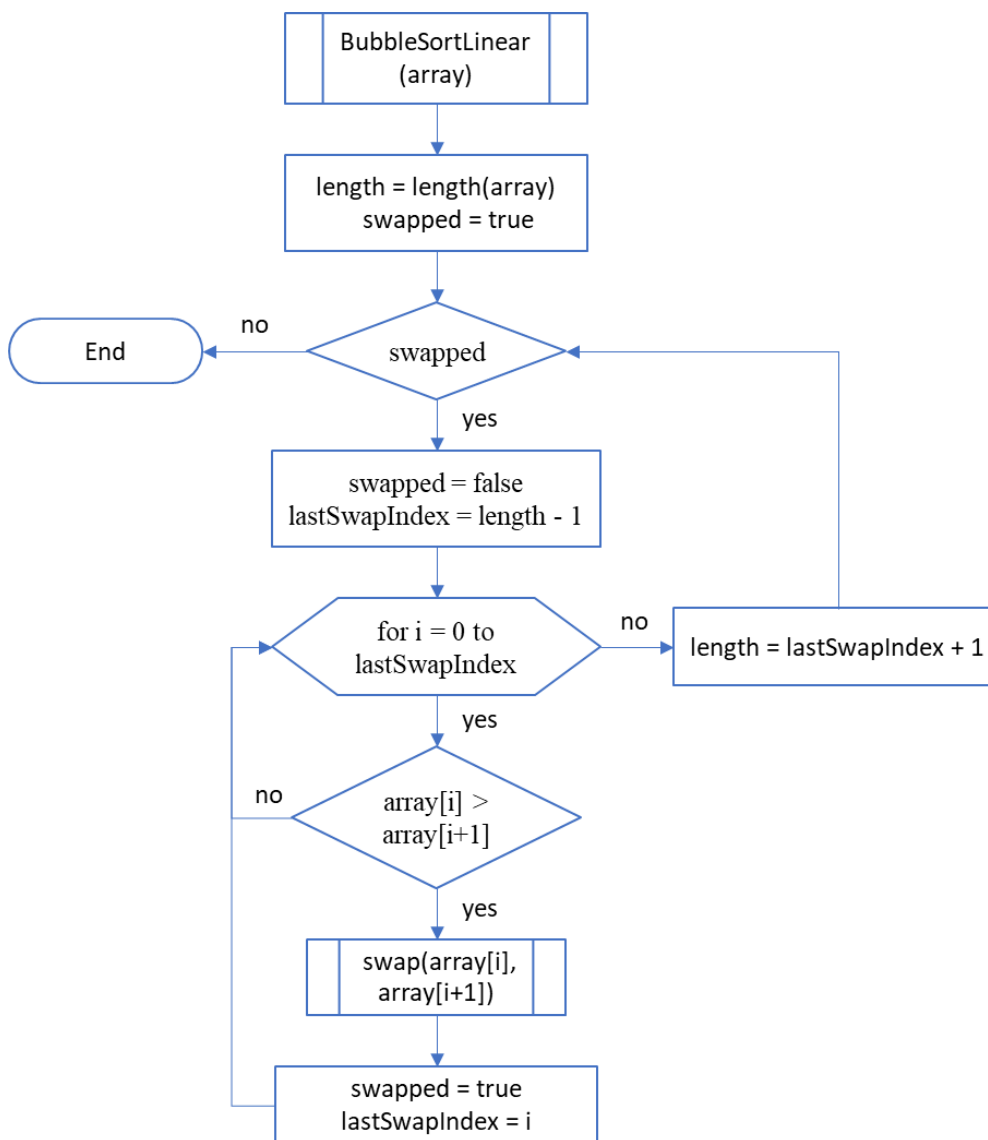
Figure 8. Flowchart of the Bubble Sort procedure
