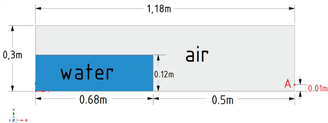
Figure 2. Test Problem Geometry
