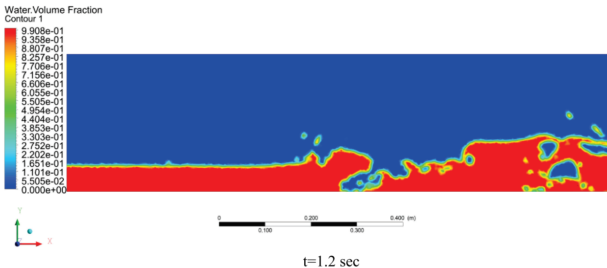
Figure 5. The contour of the change in water flow during a dam break at different times
