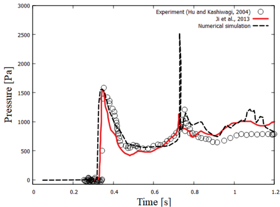
Figure 4. Water pressure for the flow during the dam break at different calculation times (0-1.2 sec).
