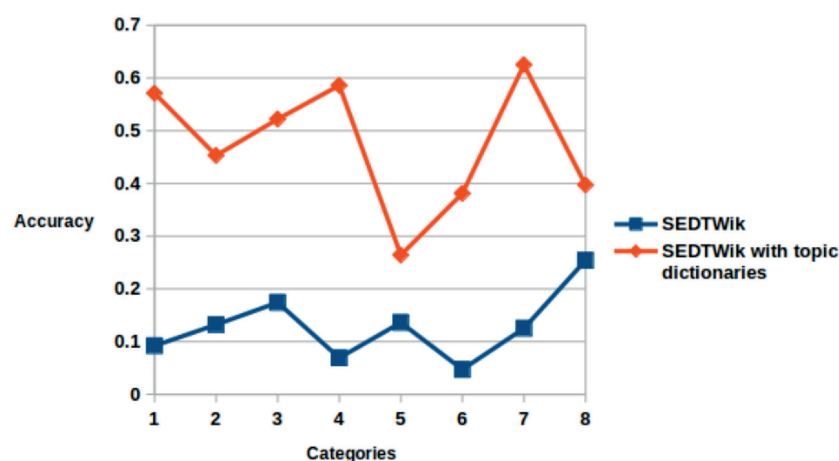
Figure 3. SEDTWik and SEDTWik with topic dictionaries accuracy
