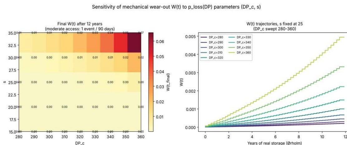
Figure 4. Sensitivity of the accumulated mechanical wear-out W(t) to the p\_loss(DP) parameters DP\_c and s , for the baseline profile under the real Ørholm climate record with a moderate synthetic access schedule.
