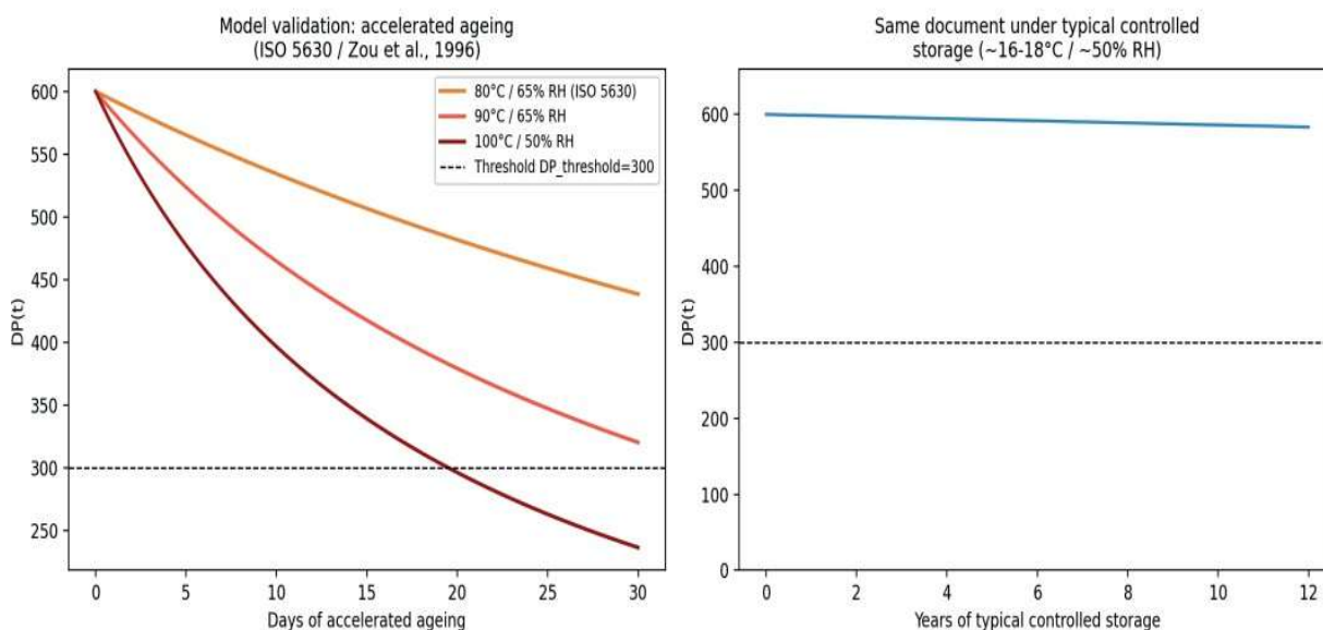
Figure 3. Model validation: the same document (pH 5, \text{DP}_0=600 ) under three accelerated-ageing regimes (left) and under typical controlled storage over 12 years (right).
